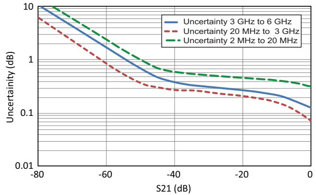
Transmission Magnitude Uncertainty
