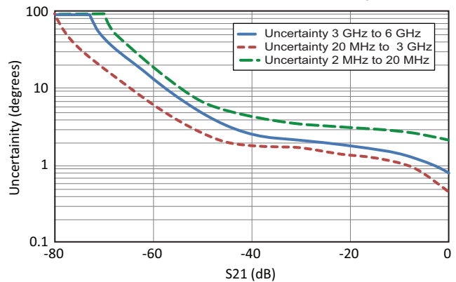
Transmission Phase Uncertainty
